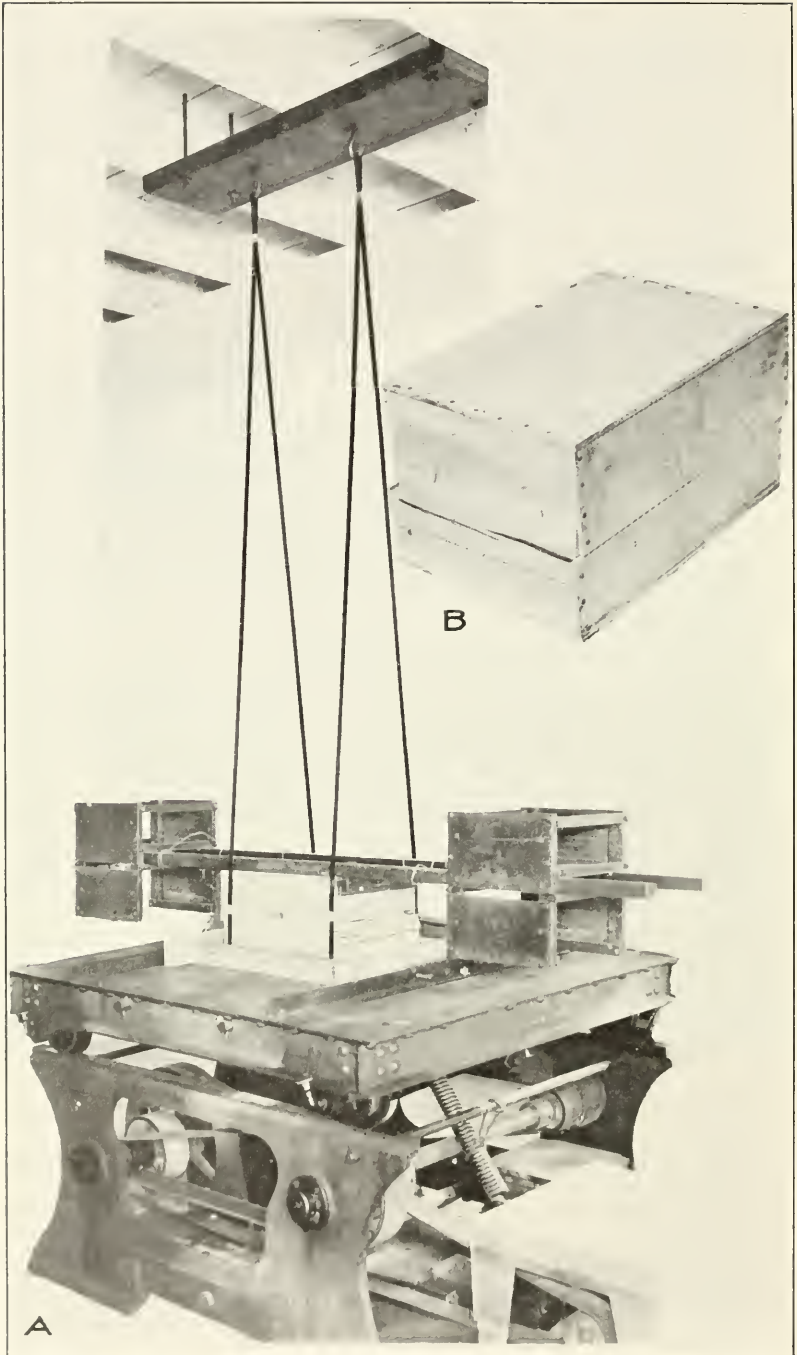
A, Oscillating table of the weening test machine adjusted for simulating the starting and stopping action of a freight car; B, box showing type of failure in this test
